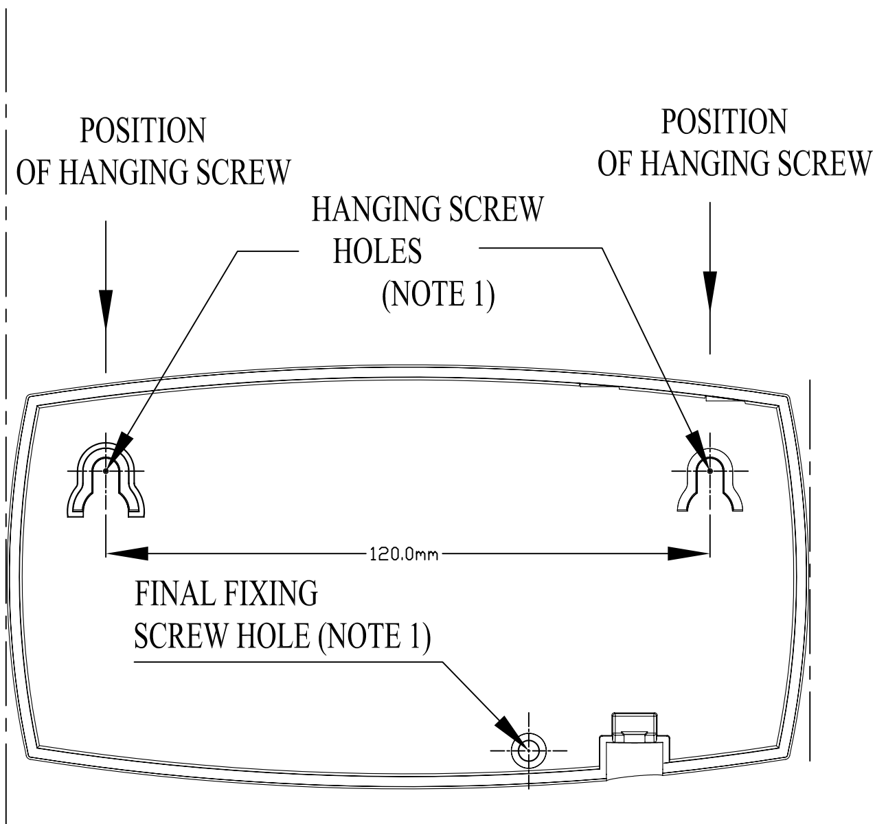
WIRED 2ZONE CONTROL PANEL MOUNTING TEMPLATE
